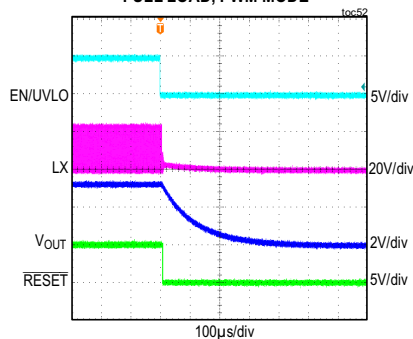
MAXM15064 SHUTDOWN THROUGH ENABLE V_{IN} = 24V , ADJUSTABLE V_{OUT} = 3.3V , FULL LOAD, PWM MODE
