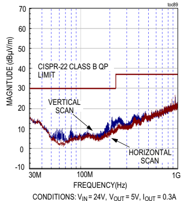
RADIATED EMISSION PLOT
