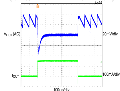
MAXM15064 LOAD TRANSIENT RESPONSE V_{IN} = 12V , ADJUSTABLE V_{OUT} = 1.5V , PFM MODE (LOAD CURRENT STEPPED FROM 5mA TO 150mA)
