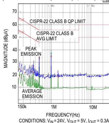
CONDUCTED EMISSION PLOT (WITH FILTER C = 0.1\mu F + 0.68\mu F , L = 82\mu H , C = 1\mu F )
