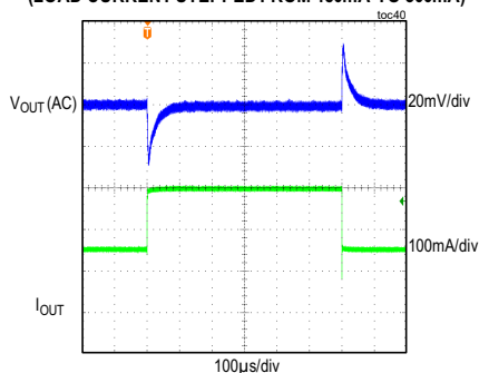
MAXM15064 LOAD TRANSIENT RESPONSE V_{IN} = 12V , ADJUSTABLE V_{OUT} = 1.5V , PFM MODE (LOAD CURRENT STEPPED FROM 150mA TO 300mA)
