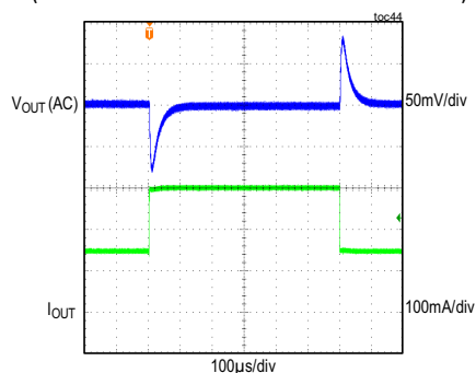
MAXM15064 LOAD TRANSIENT RESPONSE V_{IN} = 48V , ADJUSTABLE V_{OUT} = 5V , PFM MODE (LOAD CURRENT STEPPED FROM 150mA TO 300mA)
