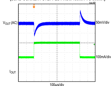
MAXM15063 LOAD TRANSIENT RESPONSE V_{IN} = 48V , FIXED V_{OUT} = 5V , PWM MODE (LOAD CURRENT STEPPED FROM 150mA TO 300mA)
