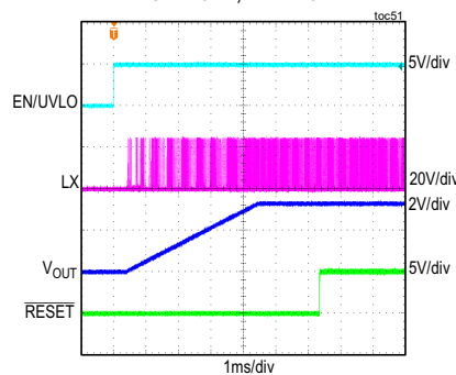
MAXM15064 STARTUP THROUGH ENABLE V_{IN} = 24V , ADJUSTABLE V_{OUT} = 3.3V , FULL LOAD, PWM MODE
