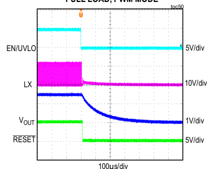
MAXM15064 SHUTDOWN THROUGH ENABLE V_{IN} = 12V , ADJUSTABLE V_{OUT} = 1.5V , FULL LOAD, PWM MODE
