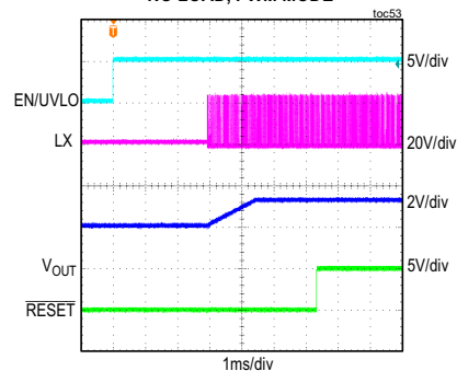
MAXM15064 STARTUP THROUGH ENABLE (2V PREBIAS) V_{IN} = 24V , ADJUSTABLE V_{OUT} = 3.3V , NO LOAD, PFM MODE
