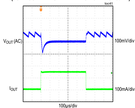
MAXM15064 LOAD TRANSIENT RESPONSE V_{IN} = 24V , ADJUSTABLE V_{OUT} = 3.3V , PFM MODE (LOAD CURRENT STEPPED FROM 5mA TO 150mA)
