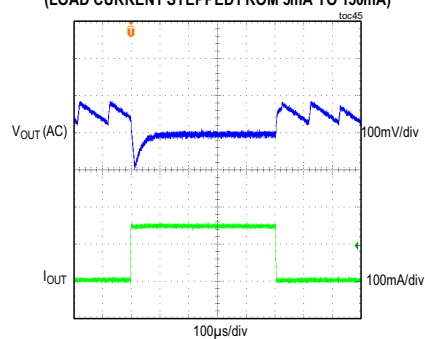
MAXM15062 LOAD TRANSIENT RESPONSE V_{IN} = 24V , FIXED V_{OUT} = 3.3V , PFM MODE (LOAD CURRENT STEPPED FROM 5mA TO 150mA)
