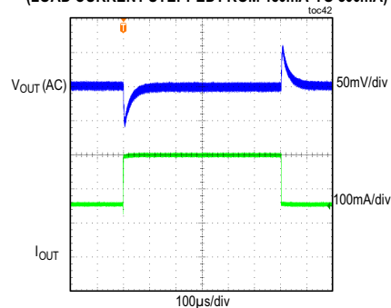
MAXM15064 LOAD TRANSIENT RESPONSE V_{IN} = 24V , ADJUSTABLE V_{OUT} = 3.3V , PFM MODE (LOAD CURRENT STEPPED FROM 150mA TO 300mA)
