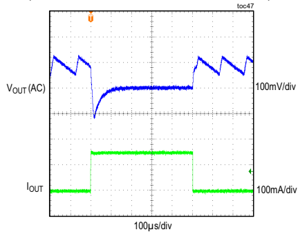
MAXM15063 LOAD TRANSIENT RESPONSE V_{IN} = 48V , FIXED V_{OUT} = 5V , PFM MODE (LOAD CURRENT STEPPED FROM 5mA TO 150mA)
