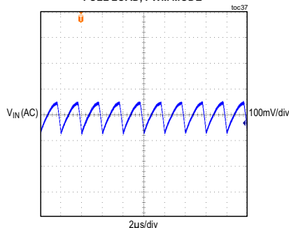
MAXM15062 INPUT VOLTAGE RIPPLE
