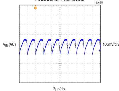
MAXM15063 INPUT VOLTAGE RIPPLE
