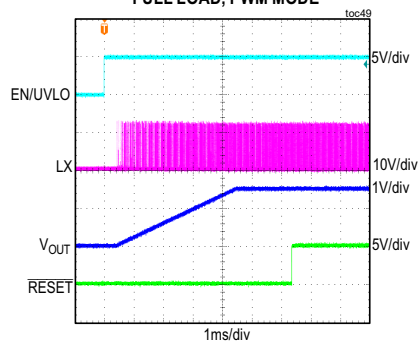
MAXM15064 STARTUP THROUGH ENABLE V_{IN} = 12V , ADJUSTABLE V_{OUT} = 1.5V , FULL LOAD, PWM MODE
